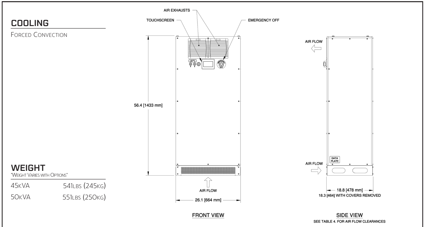
FIGURE 1 – ShorePOWER SHF 45-50kVA – F-CABINET
