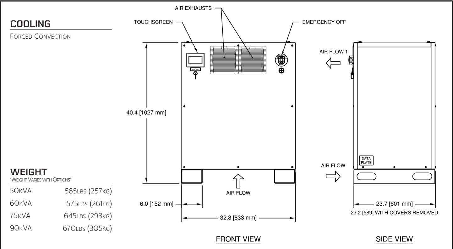
FIGURE 1 – ShorPOWER Ultra HF 50–90kVA
