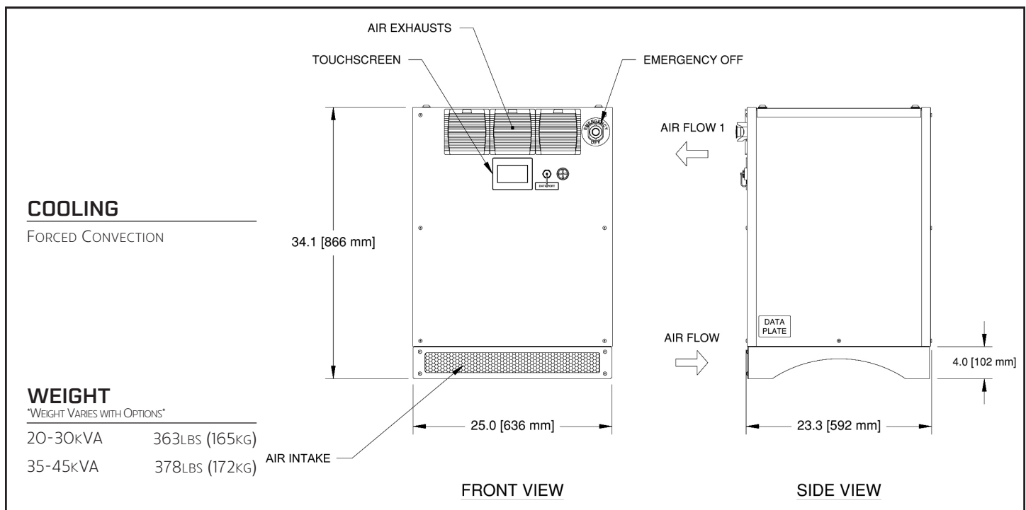
FIGURE 1 – ShorPOWER Ultra HF 20-45kVA
