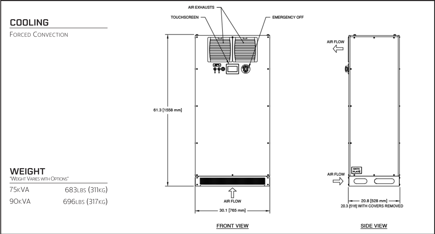
FIGURE 1 – ShorePOWER SHF 75-90kVA – F-CABINET
