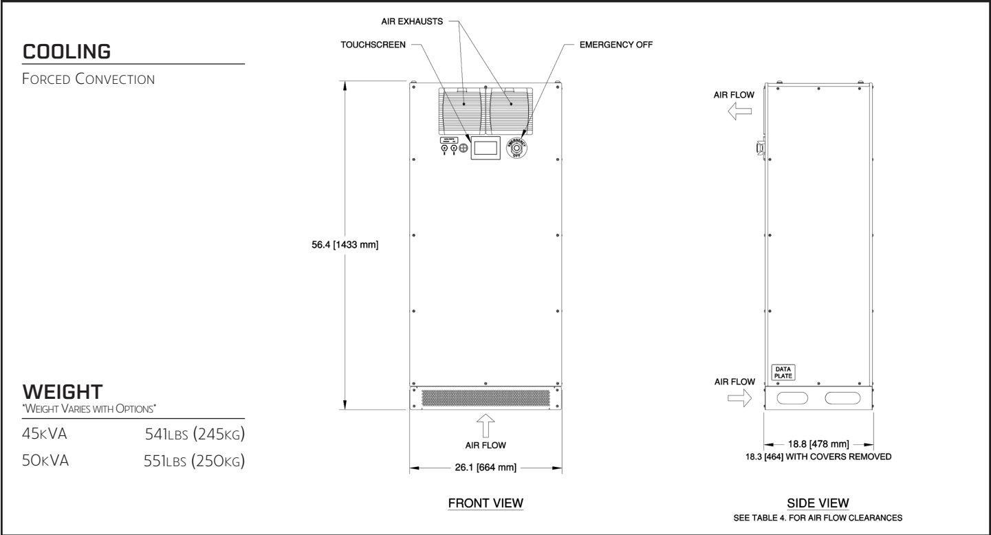
FIGURE 1 – ShorePOWER SHF 45-50kVA – F-CABINET
