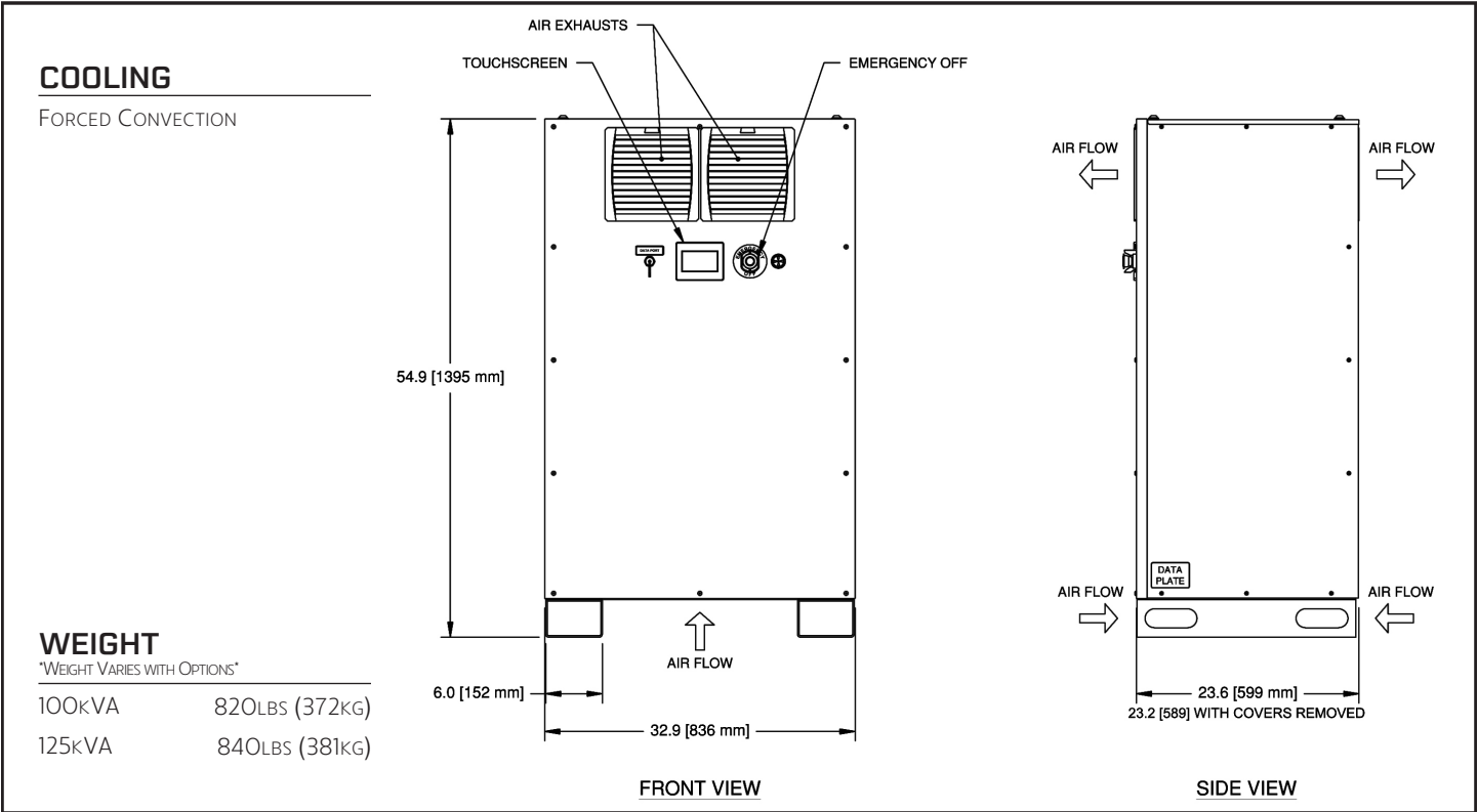
FIGURE 1 – SHORPOWER SHF 100-125kVA
